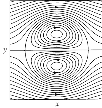
FIGURE 2. Streamlines of the Lamb–Chaplygin dipole.
